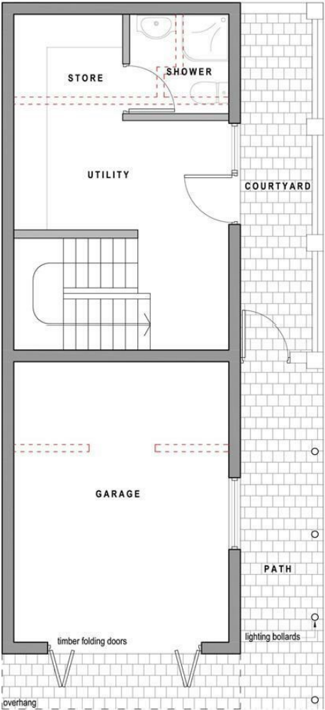
GROUND FLOOR PLAN Scale - 1:50
