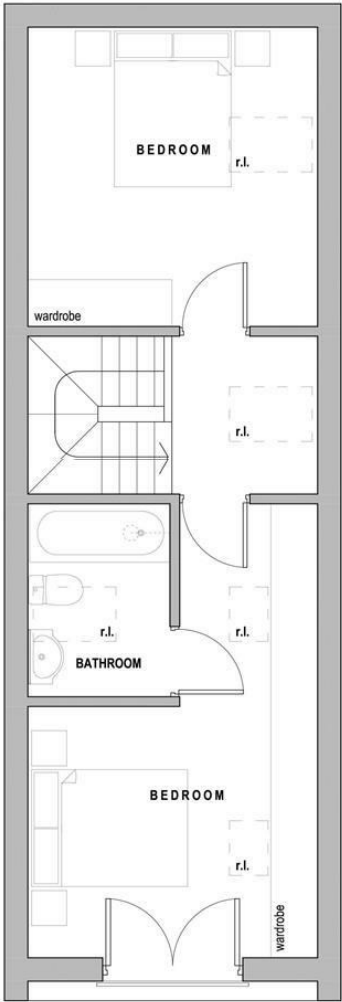
SECOND FLOOR PLAN Scale - 1:50
